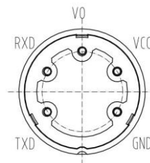
Fig3.Bottom view
