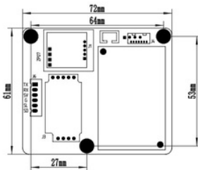
Fig 3: Mounting dimension
